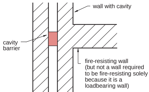
(c) Plan
