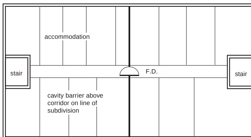
(b) Alternative arrangement plan showing subdivision of the storey by fire-resisting construction [see Table 4.6, item 7 and note (4)]
