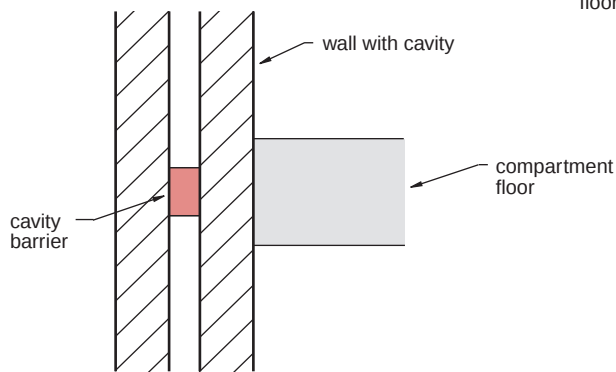
(a) Section
