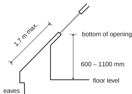
(b) Roof window (rooflight)
