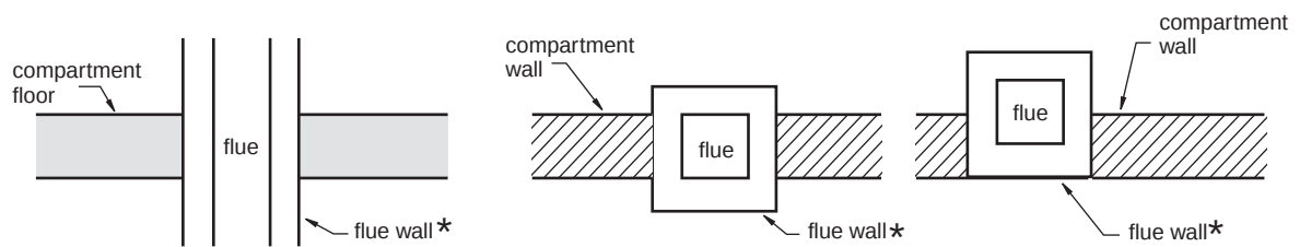
(a) Section of flue passing through a compartment floor
