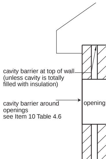
Section
