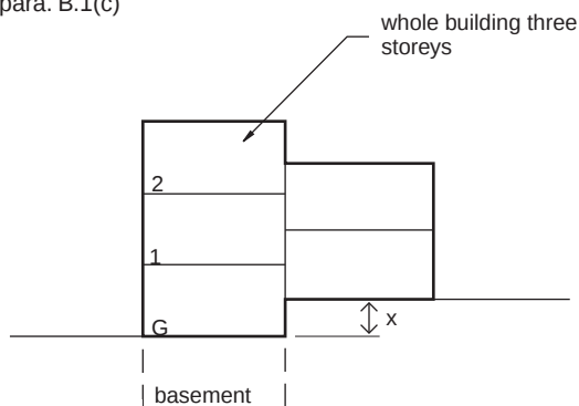
Diagram B.3 Number of storeys
