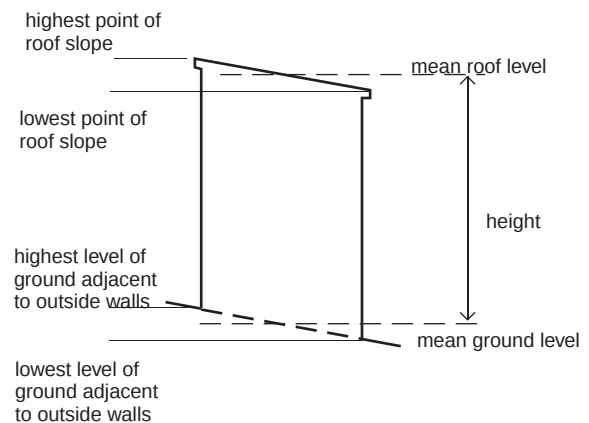
(c) Flat or monopitch roof
