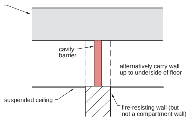
(b) Section
