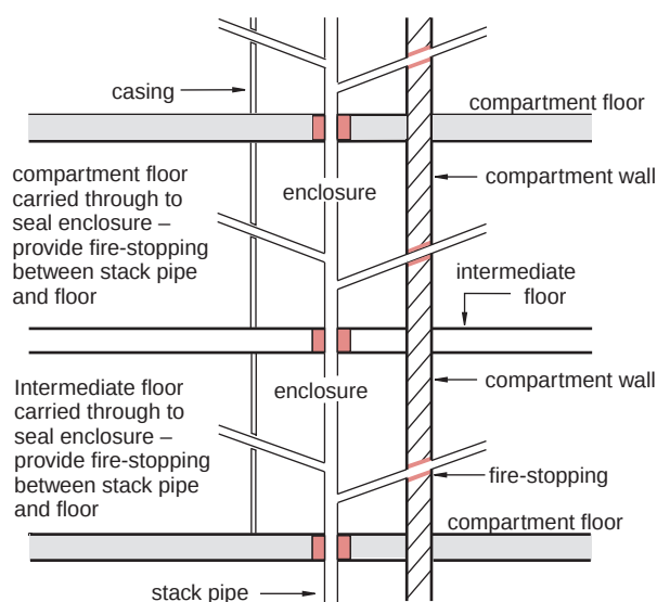
(b) Other buildings
