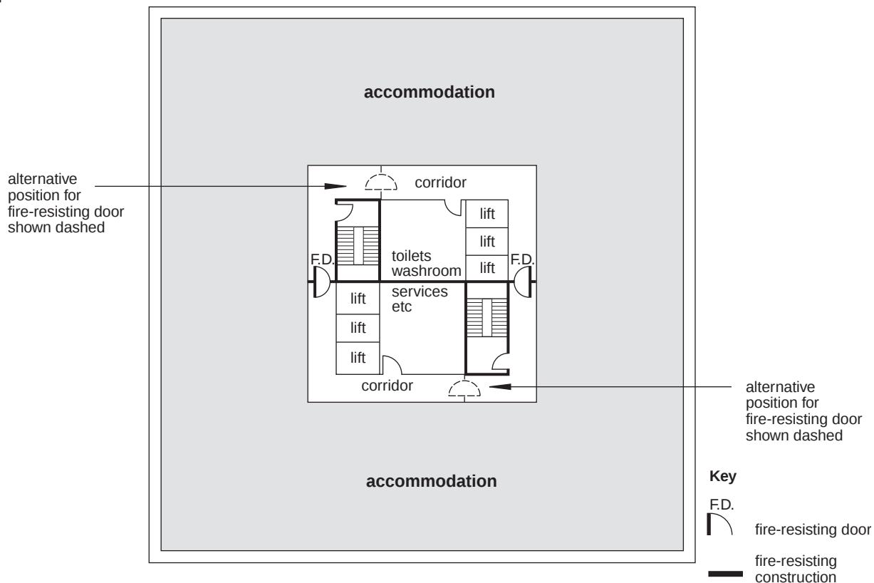
Diagram 2.8 Storey exits in a central core
