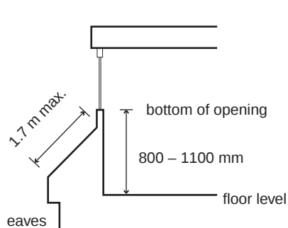
(a) Dormer window
