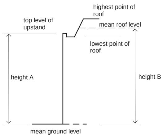
(b) Mansard type roof
