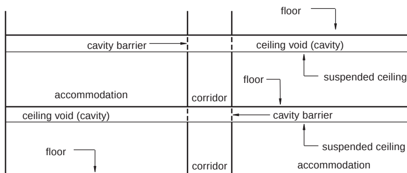
(a) Section showing use of cavity barriers above the corridor enclosure as required by Table 4.6
